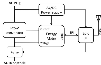
(a) ACme consists of five primary components: current-to-voltage conversion, energy metering, AC/DC power supply, microcontroller and radio, and solid state relay.
