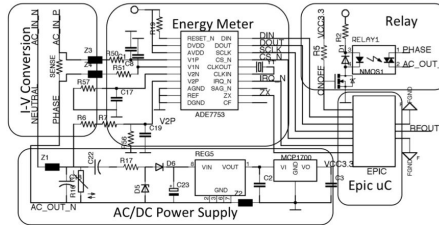
(b) ACme-A uses shunt resistor as I-V conversion, direct rectification as AC/DC power supply, and ADE7753 as the energy metering IC.
