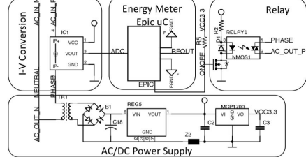
(c) ACme-B uses an in-line Hall Effect sensor as I-V conversion, a step-down transformer followed by a bridge rectifier as the AC/DC power supply, and performs energy calculation in software using the microcontroller.
